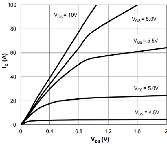
Figure 1: Saturation Characteristics
